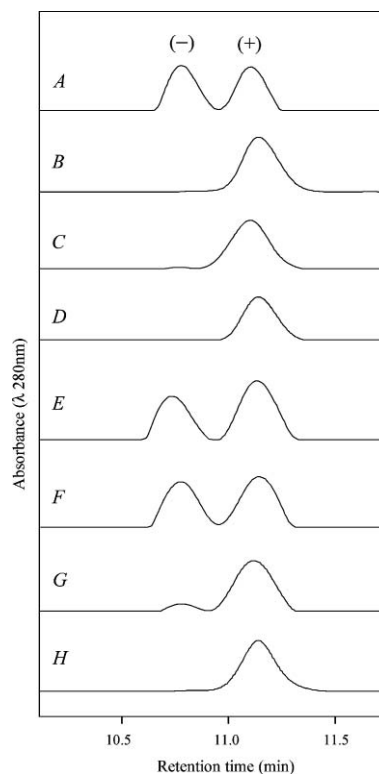
Fig. 4 The chiral HPLC chromatograms of tetrahydrohinokiresinols (THR). A, ( \pm )-THR derived from ( \pm )-EHRs. B, THR derived from ZHR, which was isolated from A. officinalis cells. C, THR derived from ZHR, which was formed by the enzymatic reaction using A. officinalis enzyme preparation. D, THR derived from ZHR, which was formed by recHRS \alpha +recHRS \beta . E, THR derived from EHR, which was formed by recHRS \alpha . F, THR derived from EHR, which was formed by recHRS \beta . G, THR derived from EHR, which was isolated from C. japonica cells. H, THR derived from EHR, which was isolated from the heartwood of C. obtusa .
