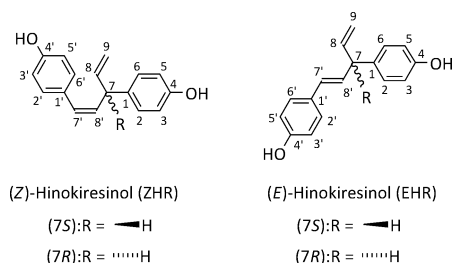
Fig. 1 The structure of hinokiresinols.
